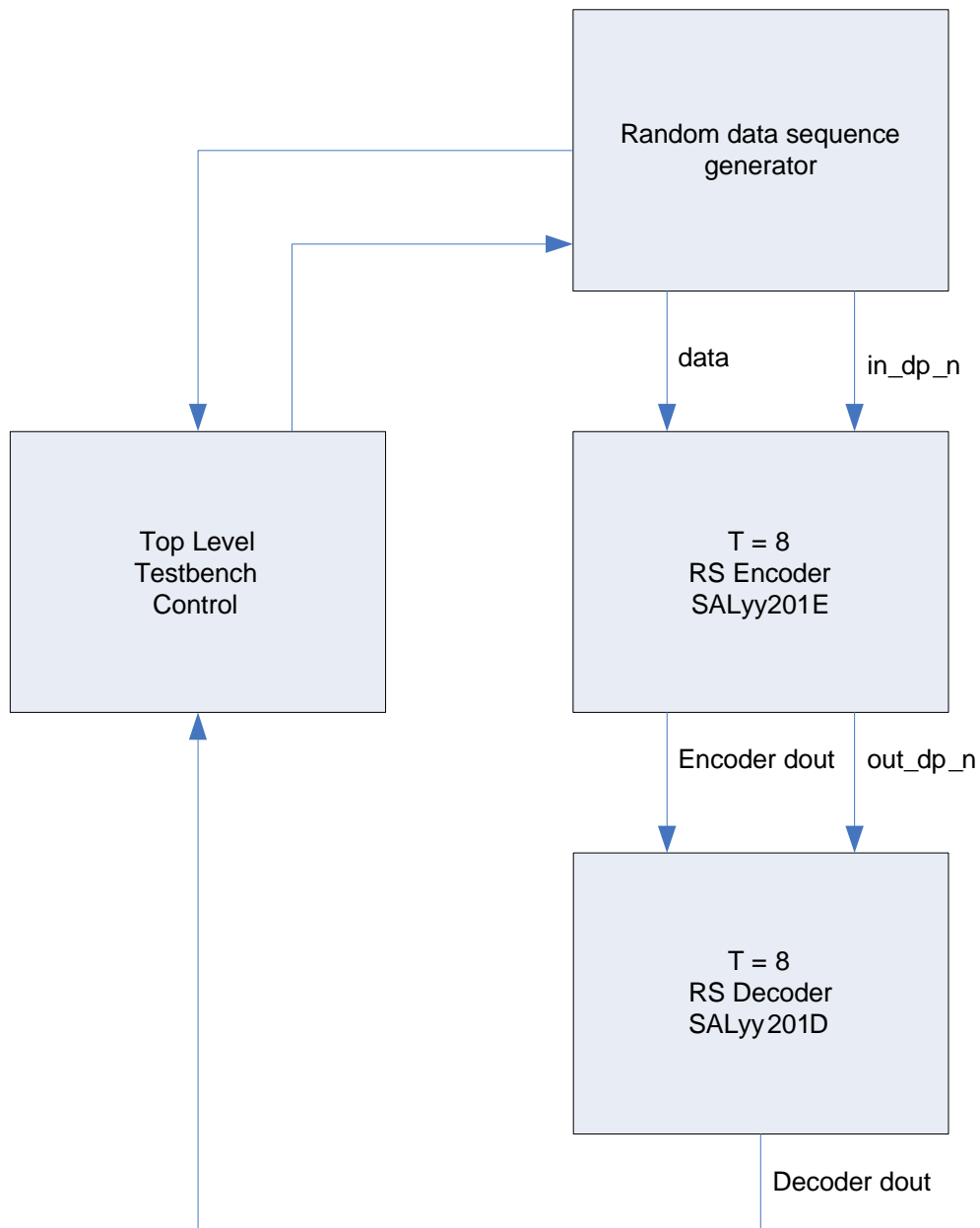
Figure 5: Testbench Block Diagram
