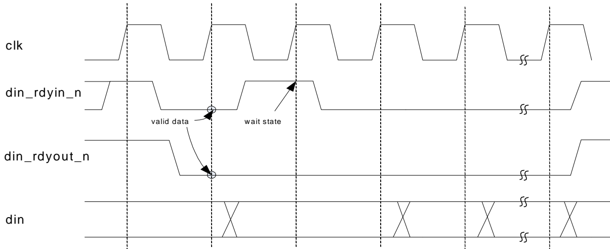
Figure 3: Input timing
