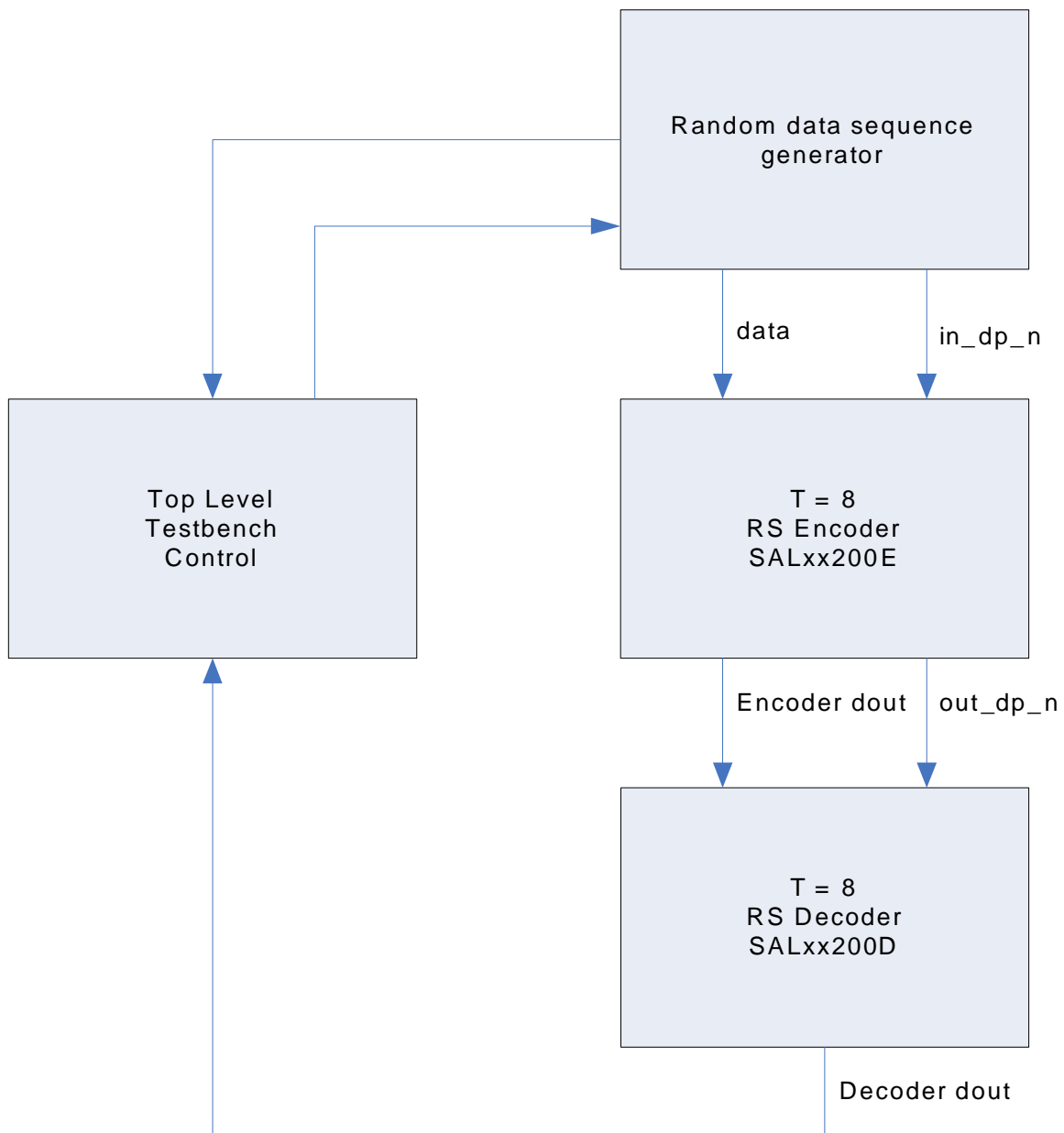
Figure 5: Testbench Block Diagram
