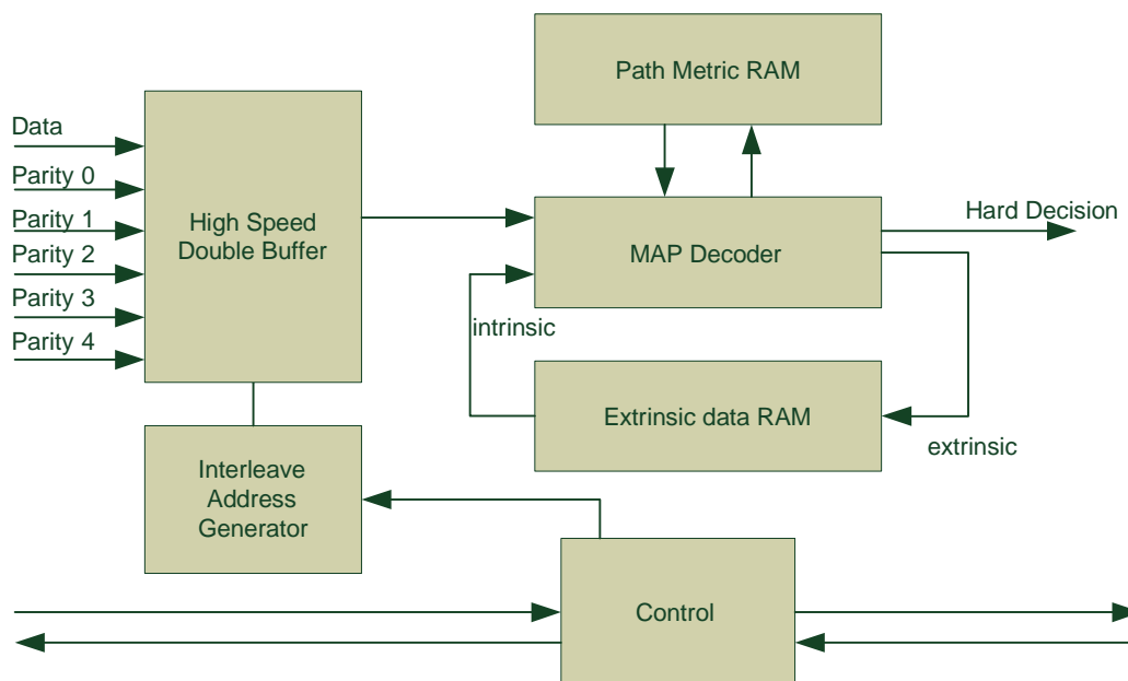
Figure 1: Decoder Block Diagram
