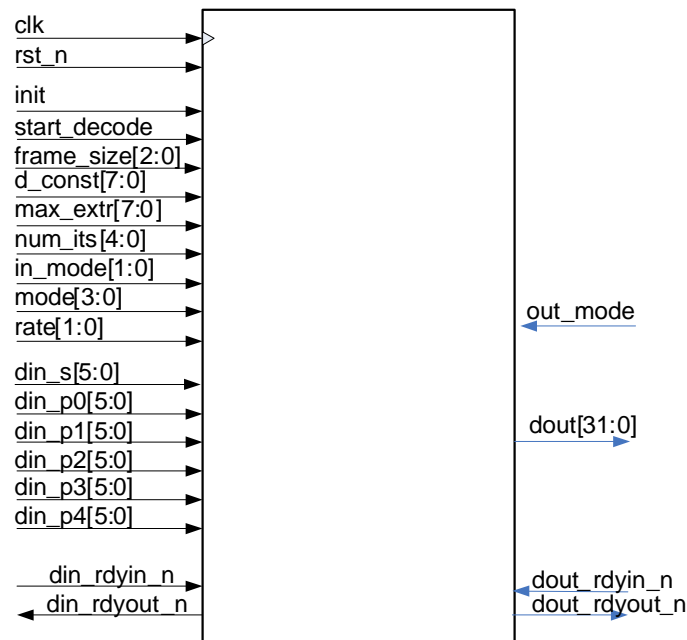
Figure 2: Component Pinout
