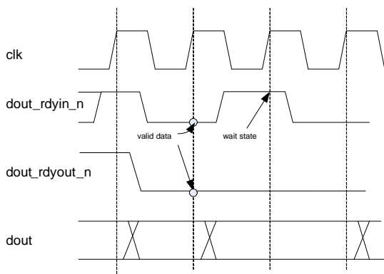
Figure 6: Output Flow Control
